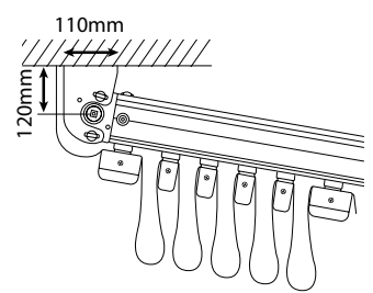
Ceiling Fixing
